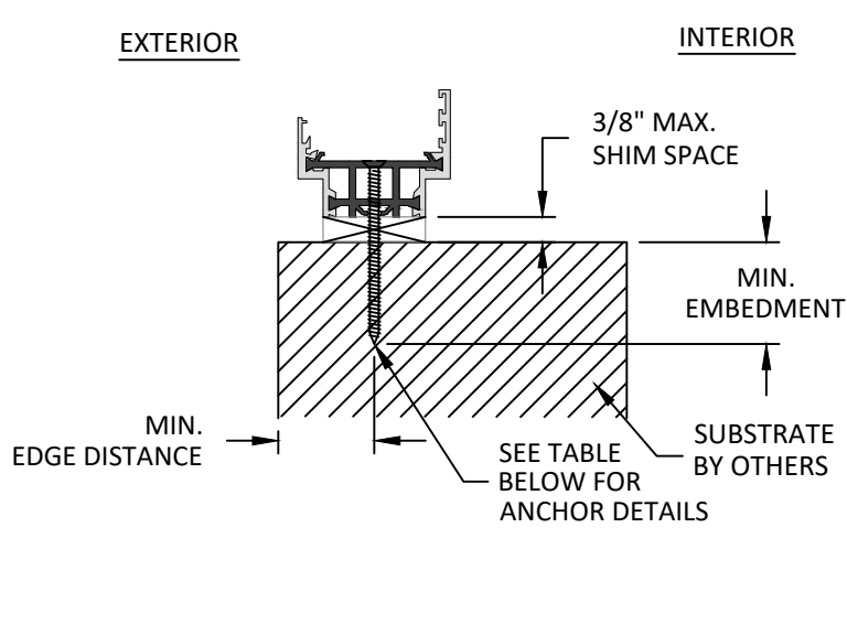
B 6 VERTICAL SECTION SILL - THROUGH FRAME
