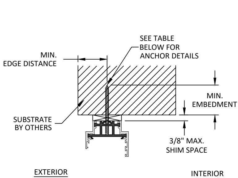
A 6 VERTICAL SECTION HEAD - THROUGH FRAME
