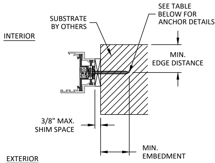
C 6 HORIZONTAL SECTION JAMB - THROUGH FRAME
